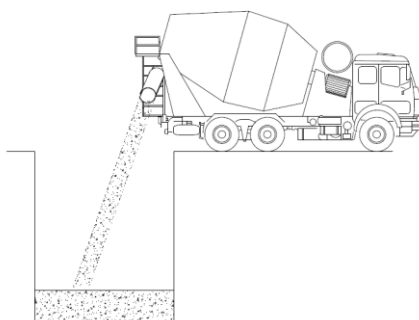
Figure 6-2 BASE CASTING
