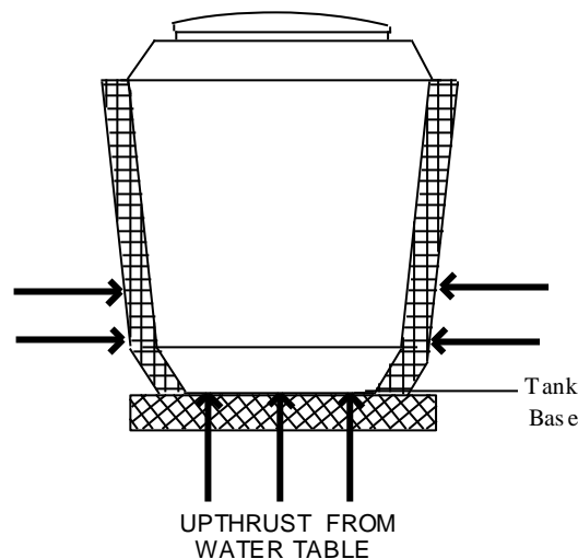
Figure 5. Pressure on HiPAF tank
