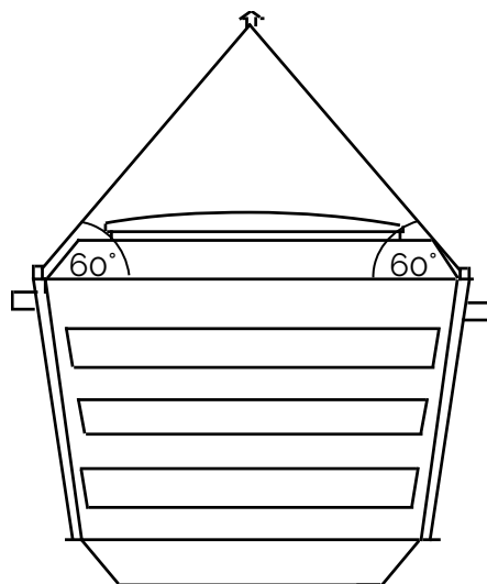
Figure 3. Correct lifting procedure
