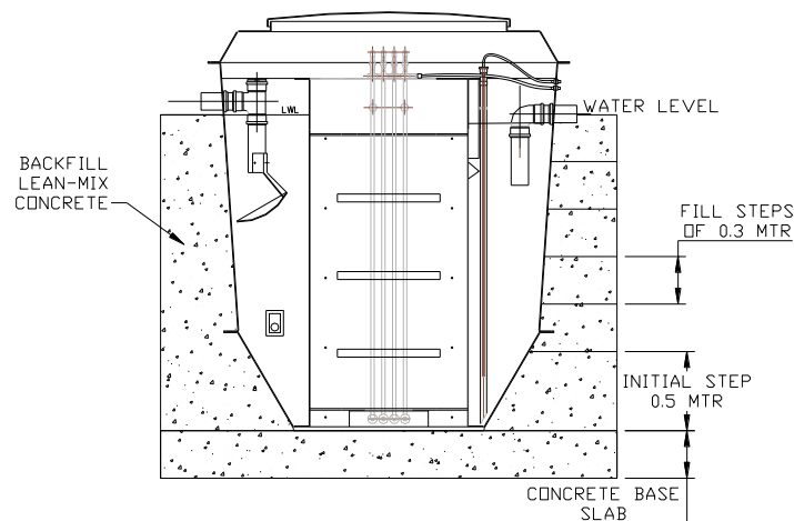
Figure 4. Concrete filling increments
