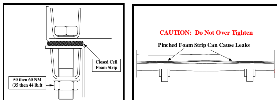
Figure 2. Bolt and Bolt Strip tightening specifications
