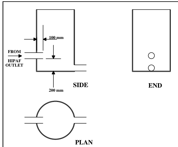
Figure 6. Sample Chamber Dimensions
